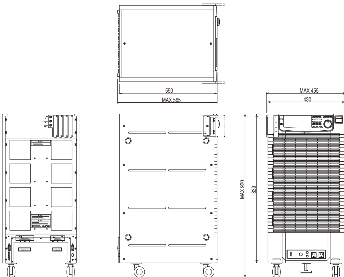
Fig. 11-8 PCR4000LA
