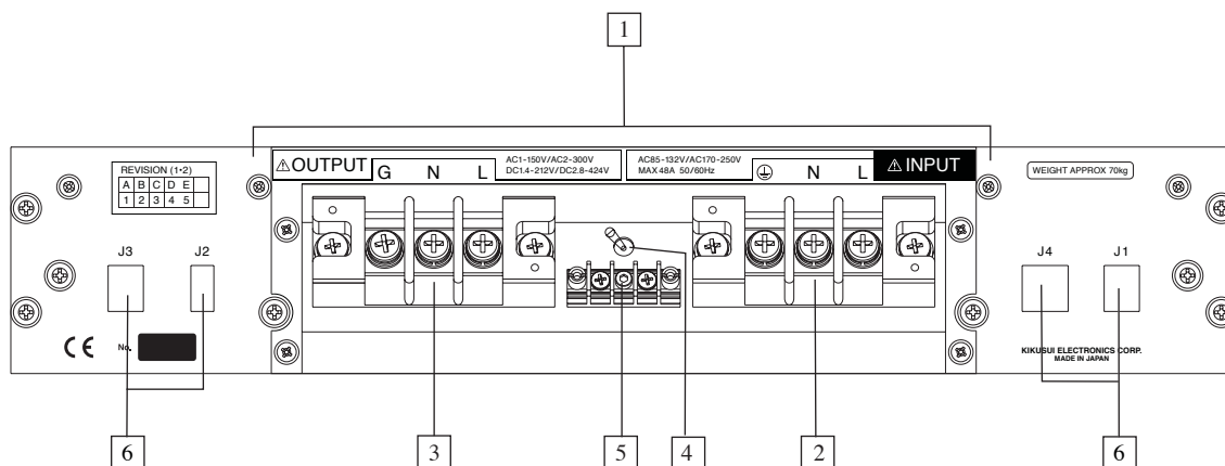
Fig. 5-13 PCR1000LA/PCR2000LA
