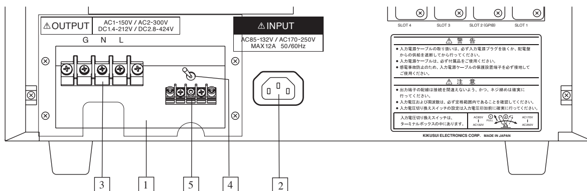
Fig. 5-12 PCR500LA
