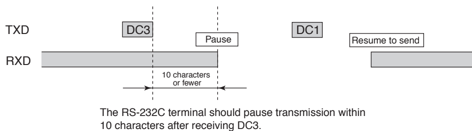
Fig.6-1 Transmission Control between the RS-232C Terminal and the PCR-LA Power Supply
