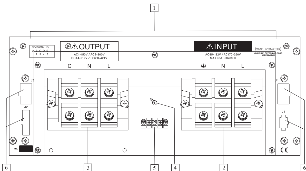
Fig. 5-14 PCR4000LA/PCR6000LA
