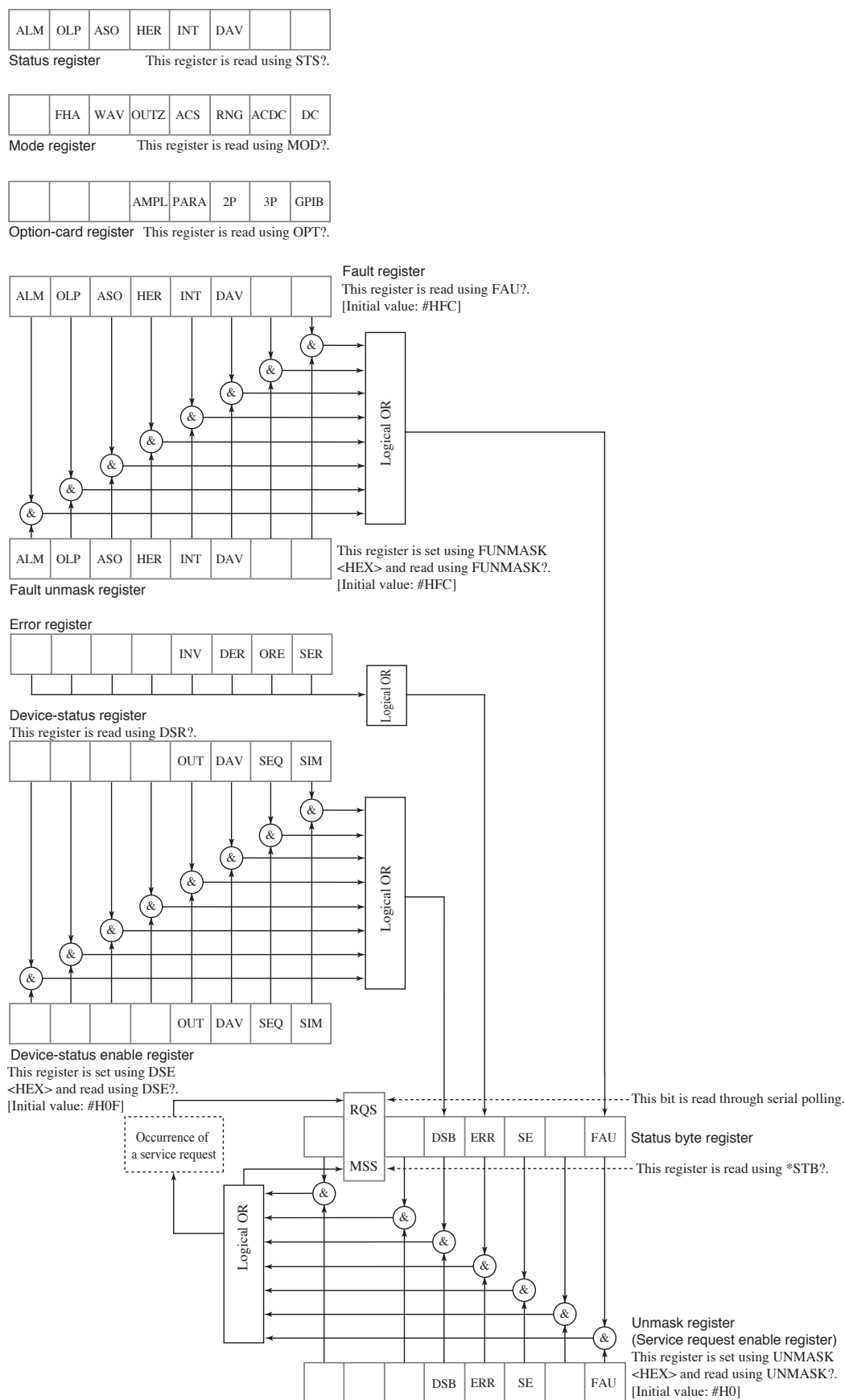
Fig. 9-5 Internal Register
